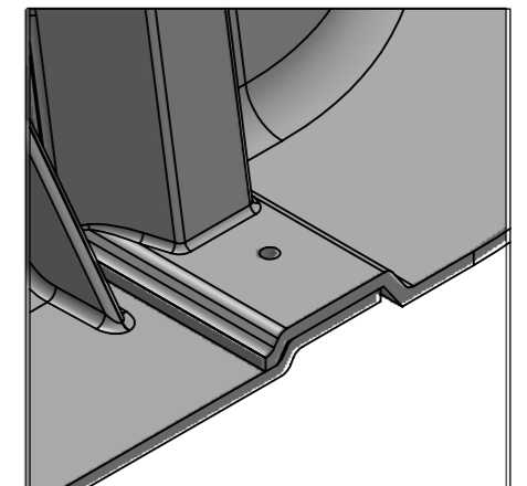
DETAIL E SCALE 1 : 4 OVERLAP AND PIN THROUGH HOLES IN BOTH PARTS
