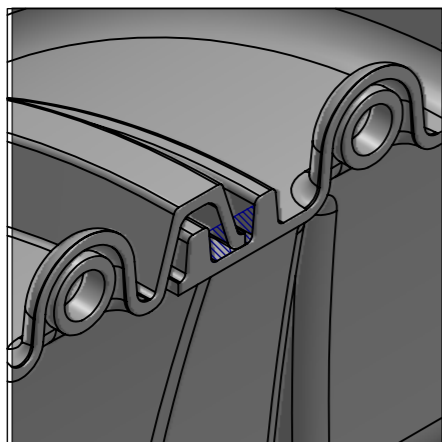
DETAIL A SCALE 1 : 4 SECTION VIEW INSERT 25 x 35mm FOAM SEALING STRIP THEN OVERLAP ARCH FEMALE LIP OVER ARCH MALE LIP
