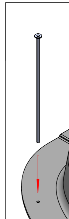
DETAIL C SCALE 1 : 8 HAMMER THE 450mm LONG PINS THROUGH THE HOLES TO SECURE THE ARCHES AND END CAPS IN POSITION
