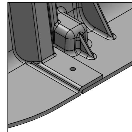
DETAIL D SCALE 1 : 4 OVERLAP AND PIN THROUGH HOLES IN BOTH PARTS
