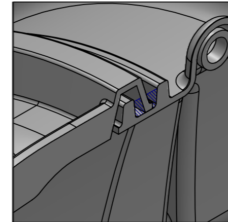
DETAIL G SCALE 1 : 4 SECTION VIEW INSERT 25 x 35mm FOAM SEALING STRIP THEN OVERLAP FEMALE END CAP OVER ARCH MALE LIP
