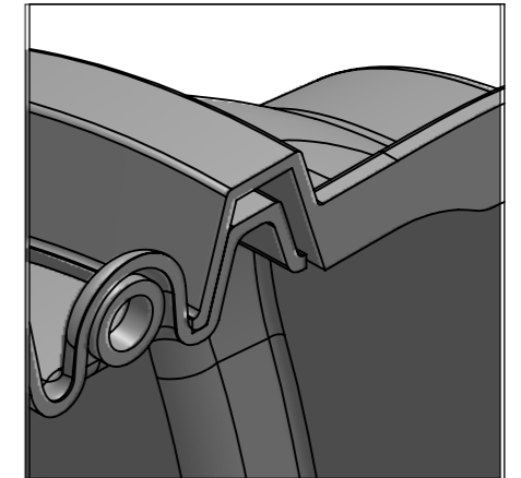
DETAIL F SCALE 1 : 4 SECTION VIEW OVERLAP MALE END CAP OVER ARCH FEMALE LIP
