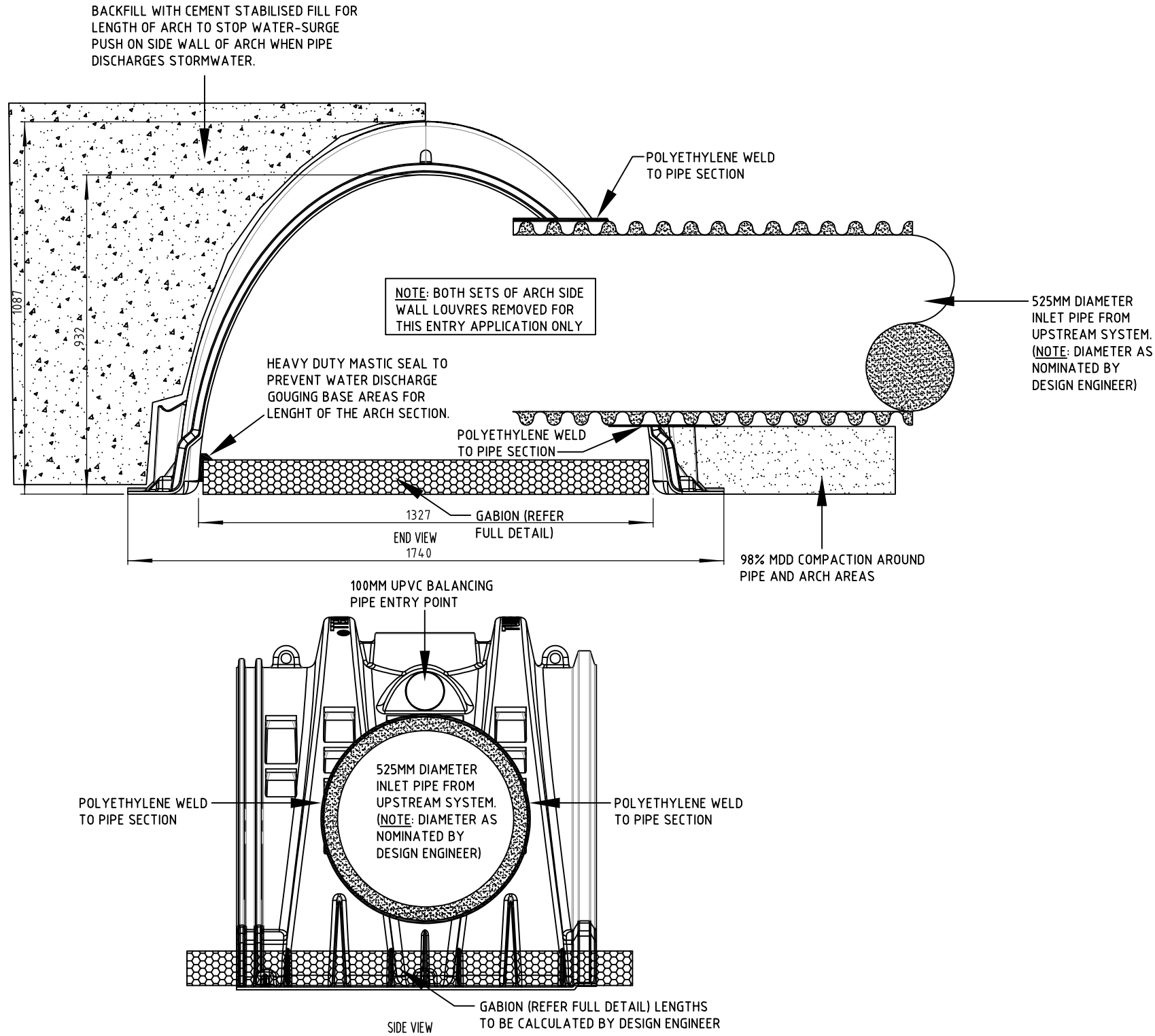
DETAIL OF LARGE PIPE - SIDE ENTRY CONNECTION - REV 0
