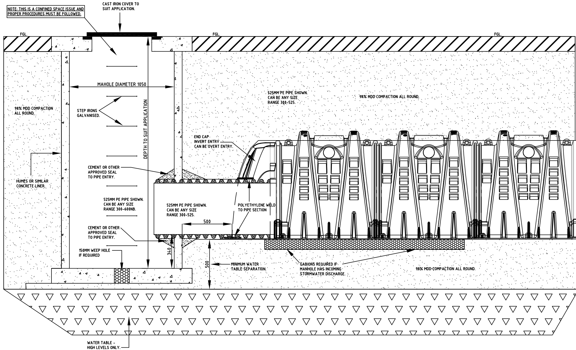
DETAIL OF INSPECTION/ACCESS CHAMBER CONNECTION - REV 0
