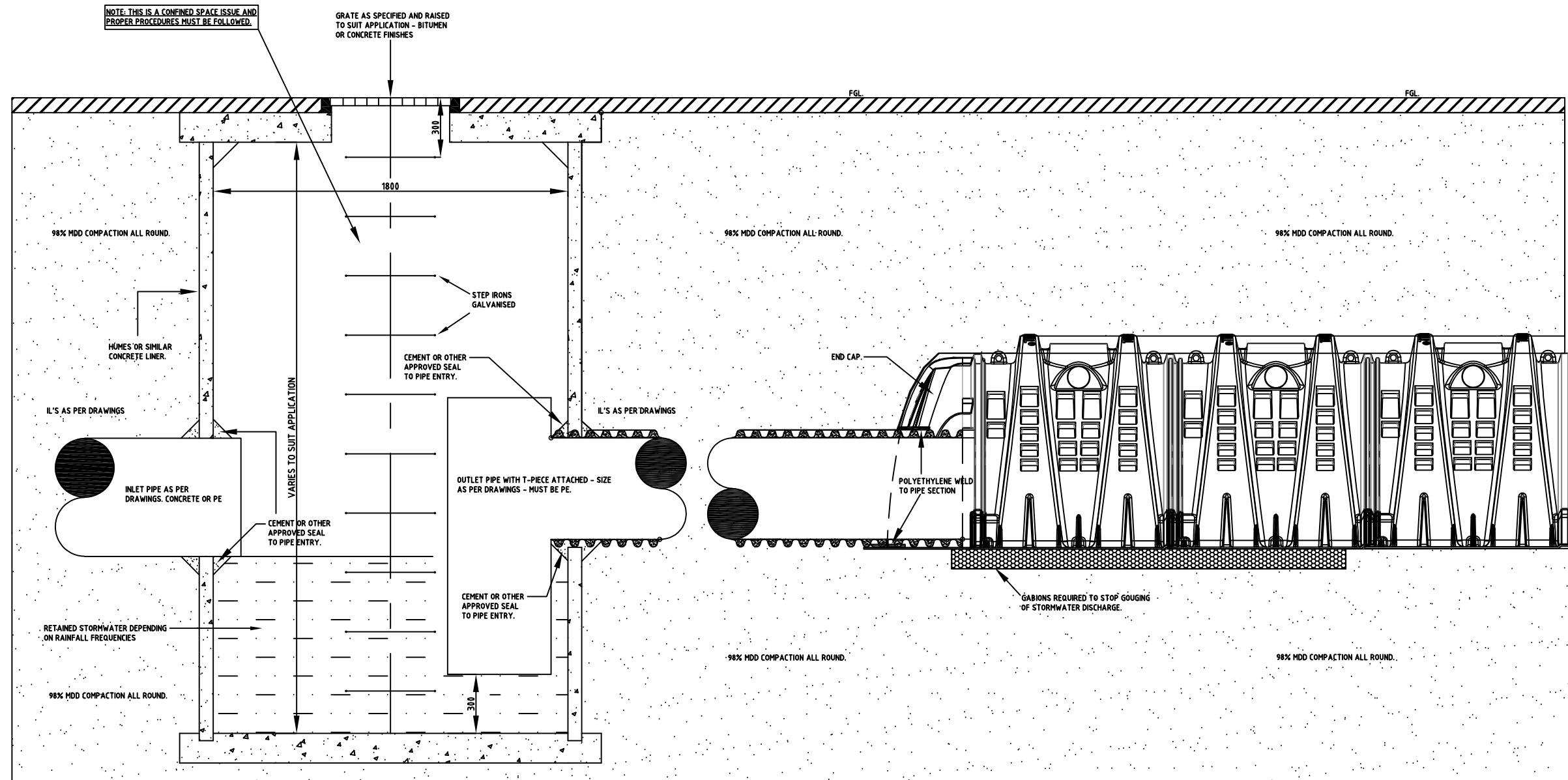
DETAIL OF DECELERATION CHAMBER CONNECTION - REV 0
